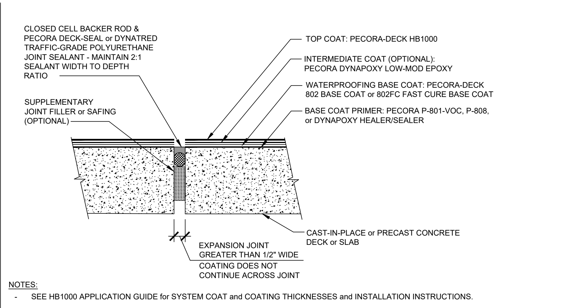
105: EXPANSION JOINTS > 1/2" WIDTH
