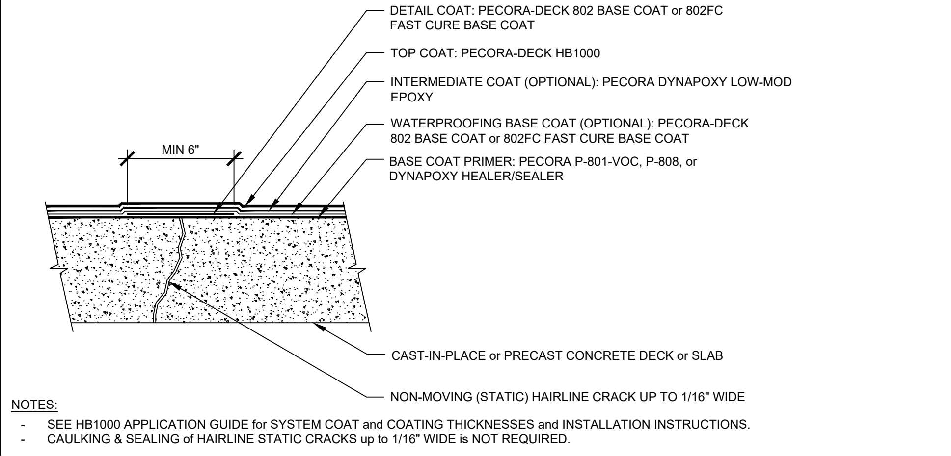
101: STATIC (HAIRLINE) CRACKS UP TO 1/16" WIDTH
