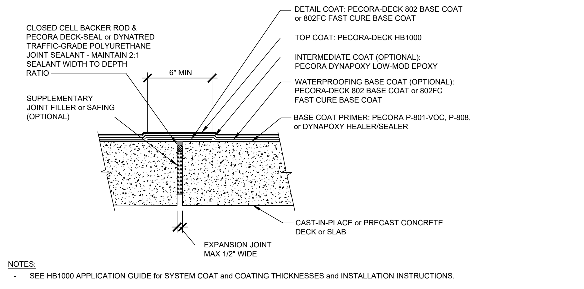
104: EXPANSION JOINTS UP TO 1/2" WIDTH
